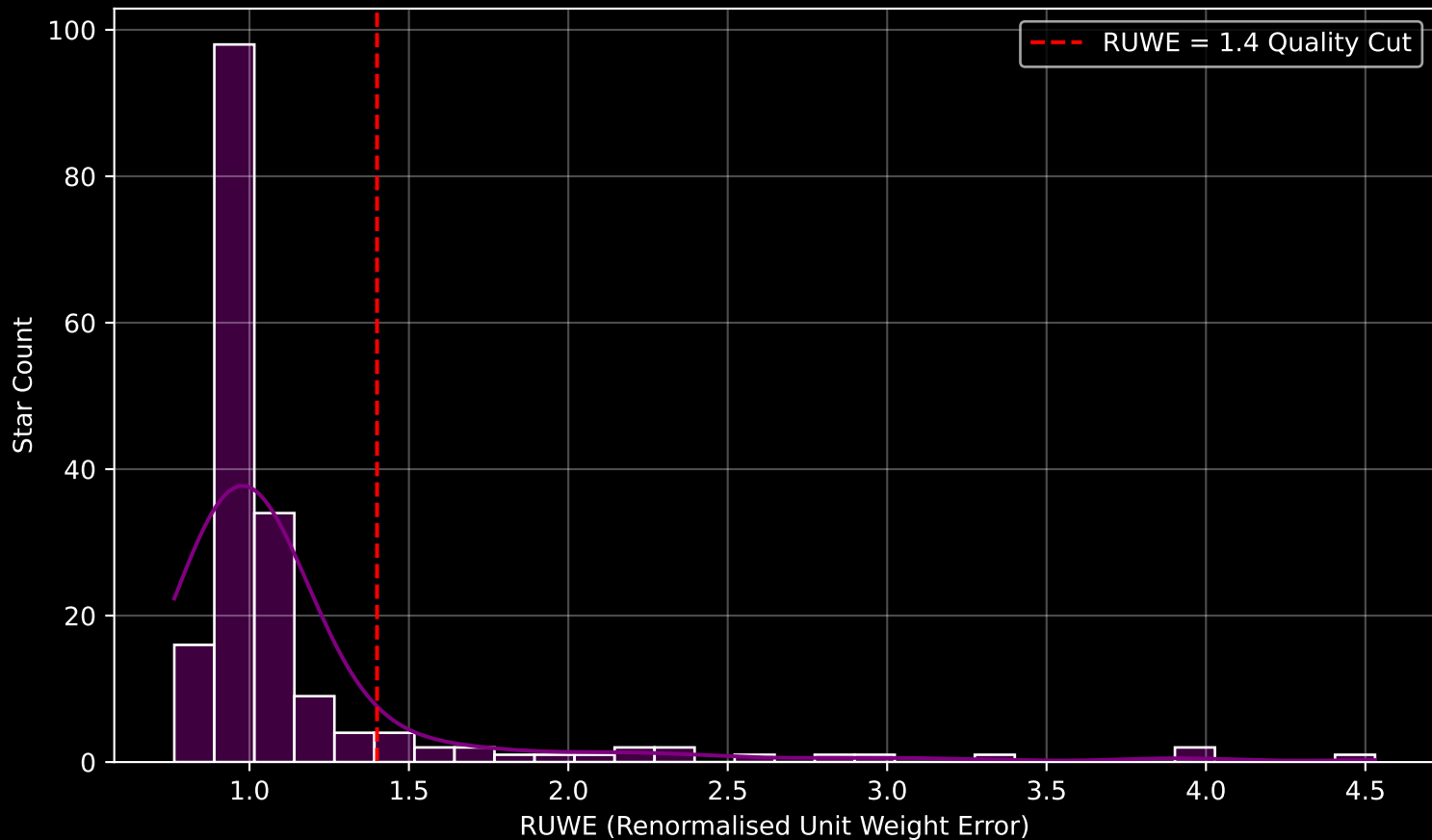
GAPOGEE DR17 Field [173+52_MGA] RUWE Distribution (n= 183)
