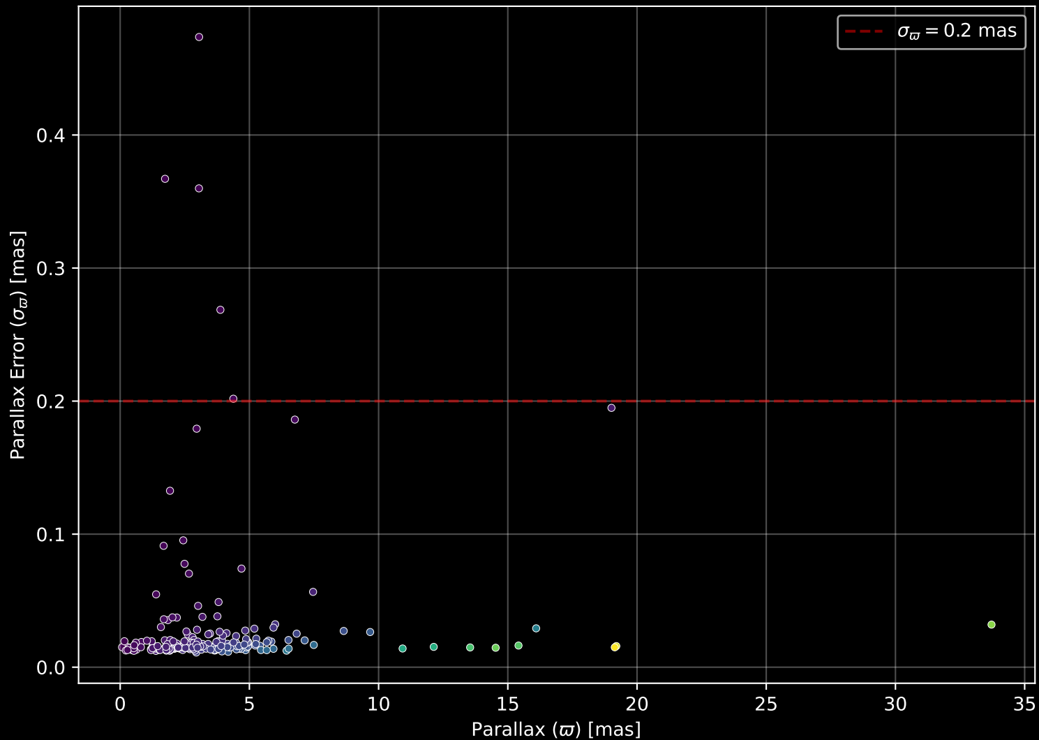
APOGEE DR17 Field: [173+52_MGA] Parallax Quality (n= 195)
