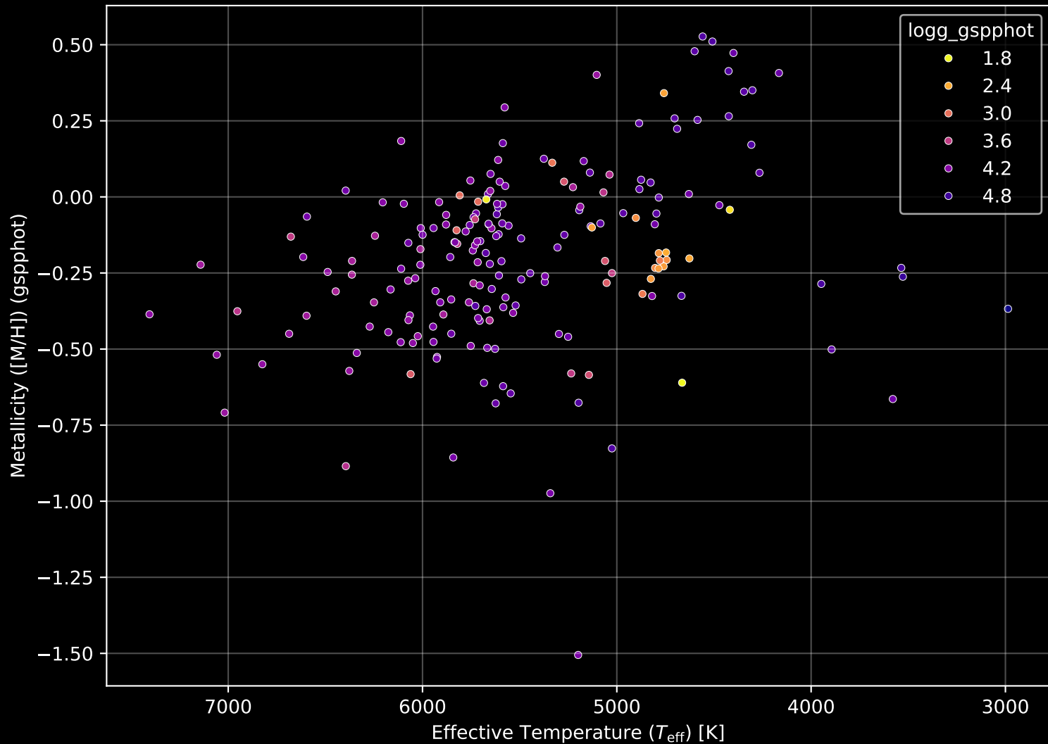
APOGEE DR17 Field: [173+52_MGA] Stellar Population Parameters (n= 195)
