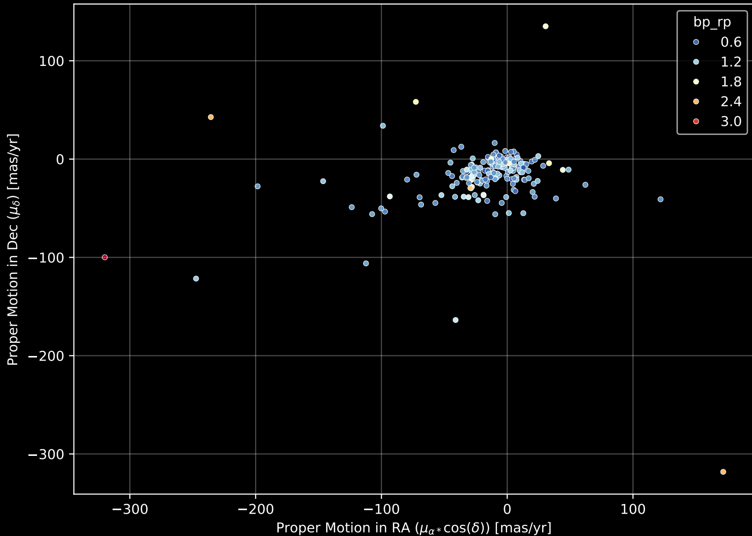
APOGEE DR17 Field: [173+52_MGA] Proper Motion Diagram (n= 195)
