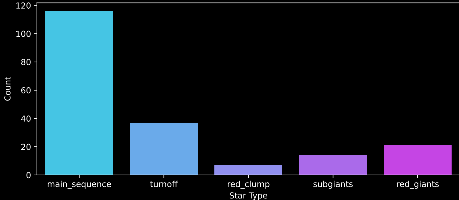
APOGEE DR17 Field: [173+52_MGA] Count plot of Star Type
