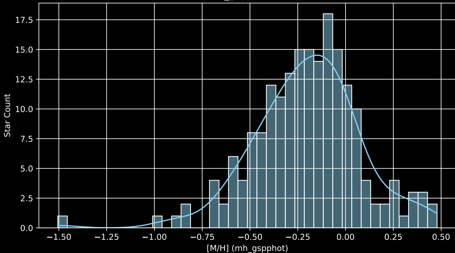
APOGEE DR17 Field: [173+52_MGA [M/H] (mh_gspphot) (n= 193)
