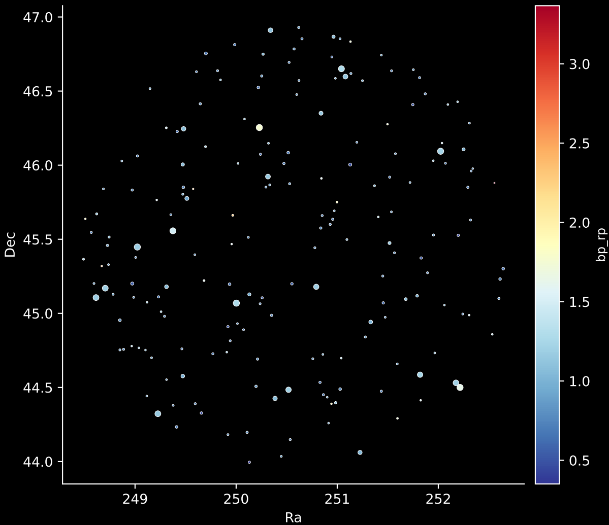
APOGEE DR17 Field: [173+52_MGA] Stars: 195
